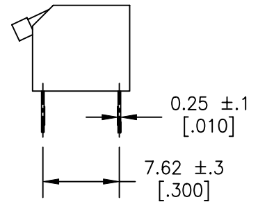
SRPG202S1B SHOWN
